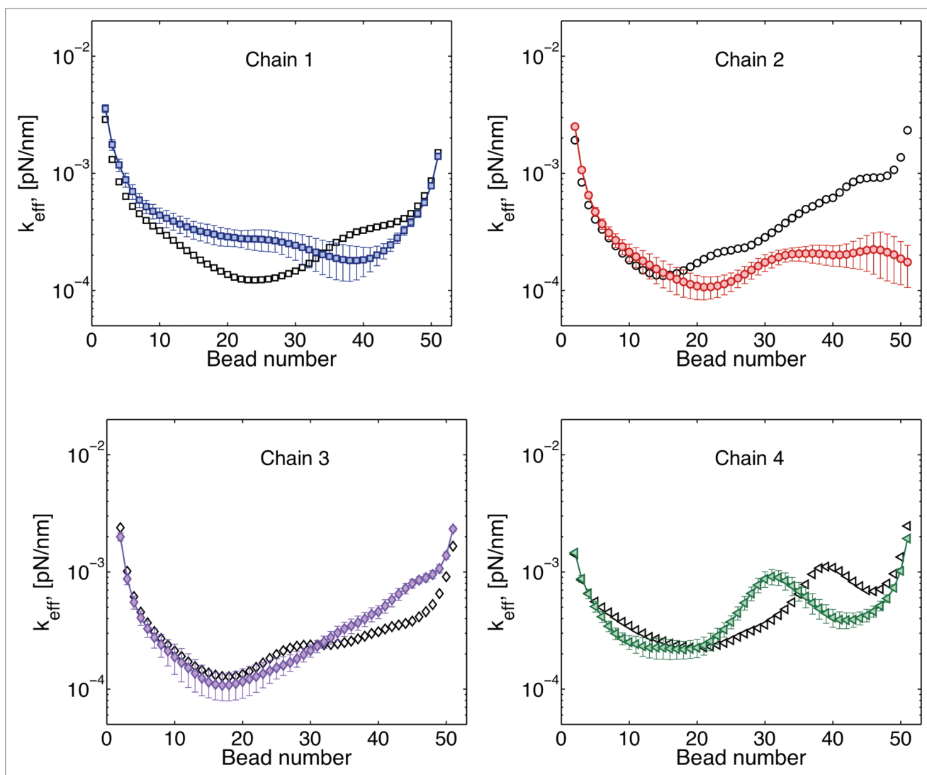
Figure 12. Effective spring constant after the telomere site of chain 2 becomes untethered. Black symbols correspond to results where all the chains are tethered at both ends. Color symbols correspond to the resulting behavior for the free motion of the telomere site of chain 2. Motion at the telomere end in chain 2 is increased, while motion of other chains might increase or decrease depending of the location within the chain. Similar behavior is obtained when the telomere site of other chains is allowed to move freely.
