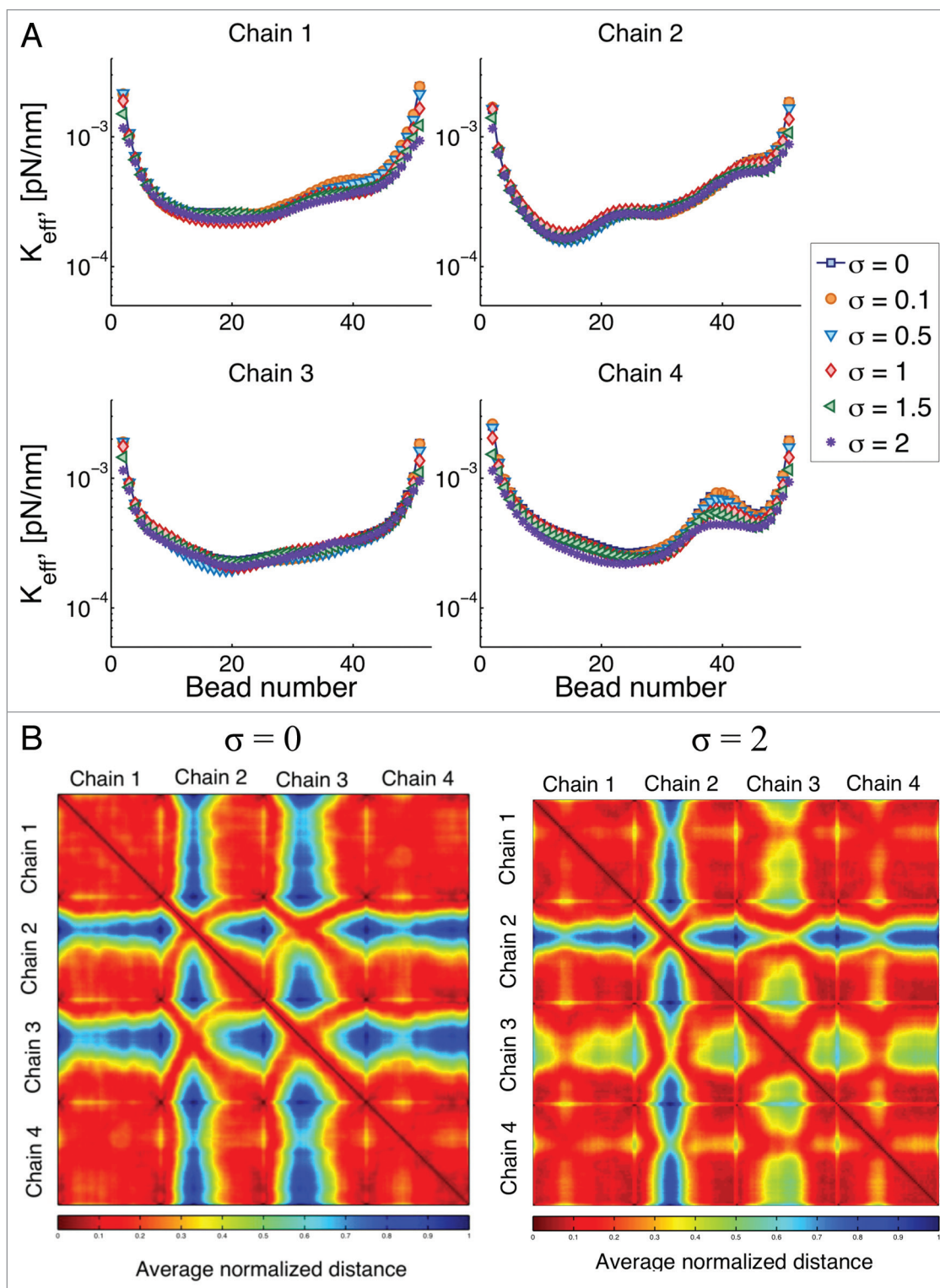
Figure 8. (A) Effective spring constant for different type of interactions with the confining wall. After a bead leaves the simulation domain (circle of radius 1 micron) the probability of coming back to the confining boundary is Gaussian, with standard deviation \sigma . So that if \sigma = 0 the boundary is a “hard-wall”, and as \sigma increases the “softness” of the wall increases. (B) Interaction heat maps for hard and soft walls.
