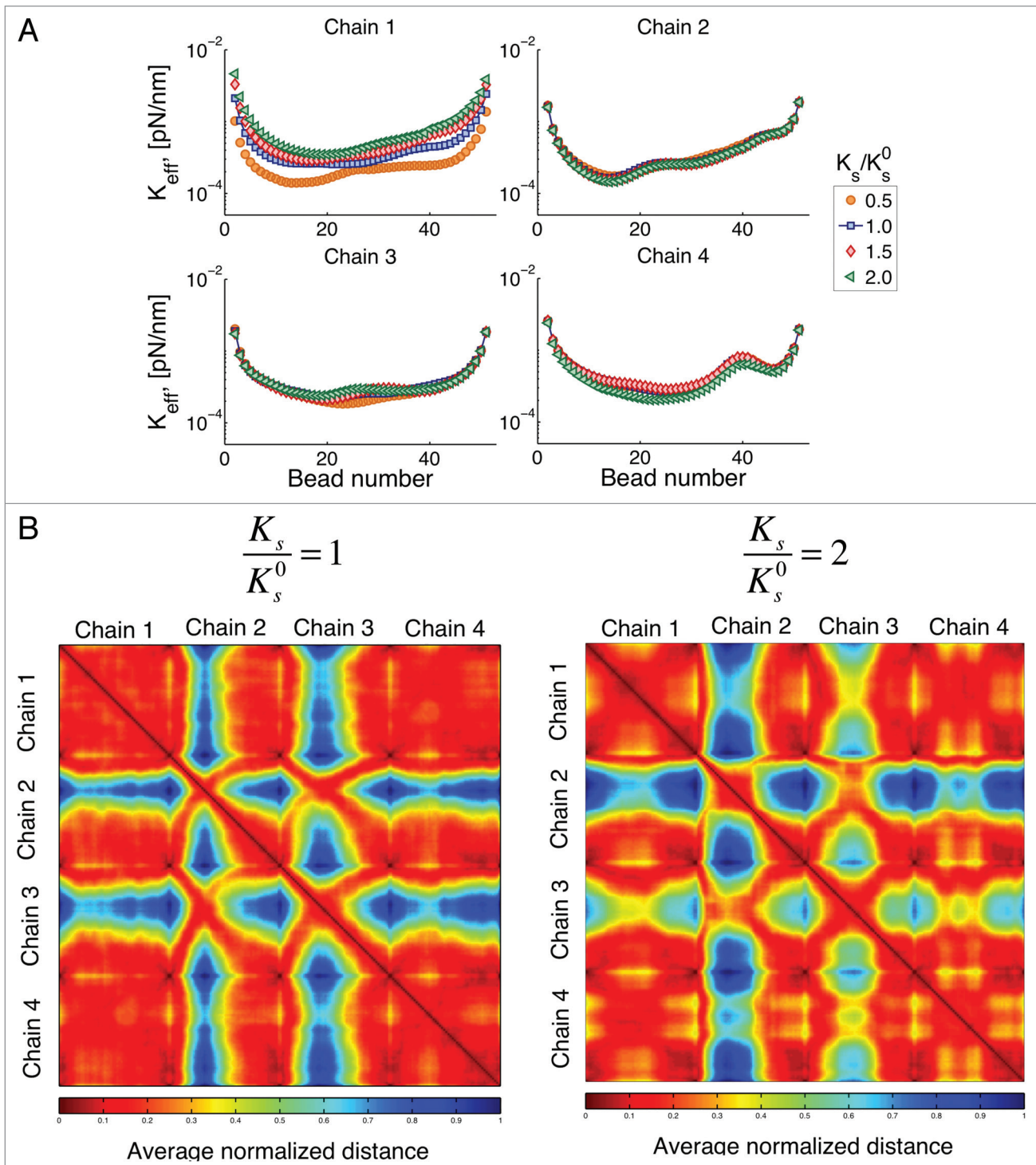
Figure 10. (A) Effective spring constant for variations of stiffness of chain 1. K_s is the spring constant for chain 1, K_s^0 is the spring constant for other chains obtained using Eqn. (3) and L_p = 50 nm. Changes of the properties of one chain affects the behavior of other chains through changes in their interactions. (B) Interaction heat maps for two different values of K_s . If chain 1 is stiffer, interaction of chain 2 with other chains is reduced, while interactions between chains 3 with other chains is increased. This figure shows how changes of the properties on a single chain, can affect the behavior of the whole system (global response to local changes). Similar behavior is observed if we choose to change the spring constant of any other chain.
