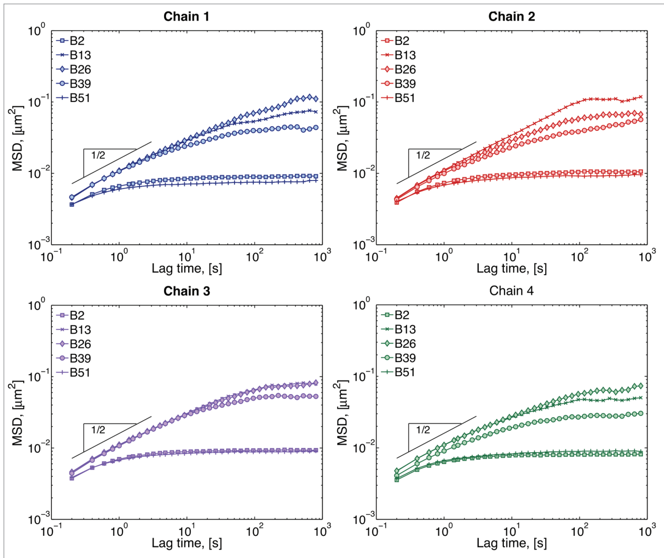
Figure 3. Mean-squared displacement (MSD) of selected beads within each chain. Short-lag time behavior is sub-diffusive, while the plateau at large lag times comes from the confinement of the nucleus wall and tethering of the chains. The inverse of the plateau value gives an approximation of the range of motion of the beads. 26 Beads close to the tethers explore smaller spaces than beads in the middle of the chain.
