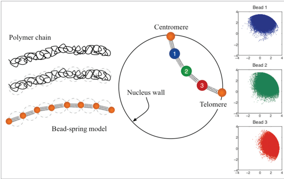
Figure 2. Coarse-grained representation of chromosome arms using bead-spring models. Since entropy is proportional to the log of the number of the microscopic states; 32 in this model the entropy comes from the number of possible configurations. Configuration space is then a function of the number of beads, the spring constant of the individual springs, the confinement of the nucleus wall, and the excluded volume interactions.
