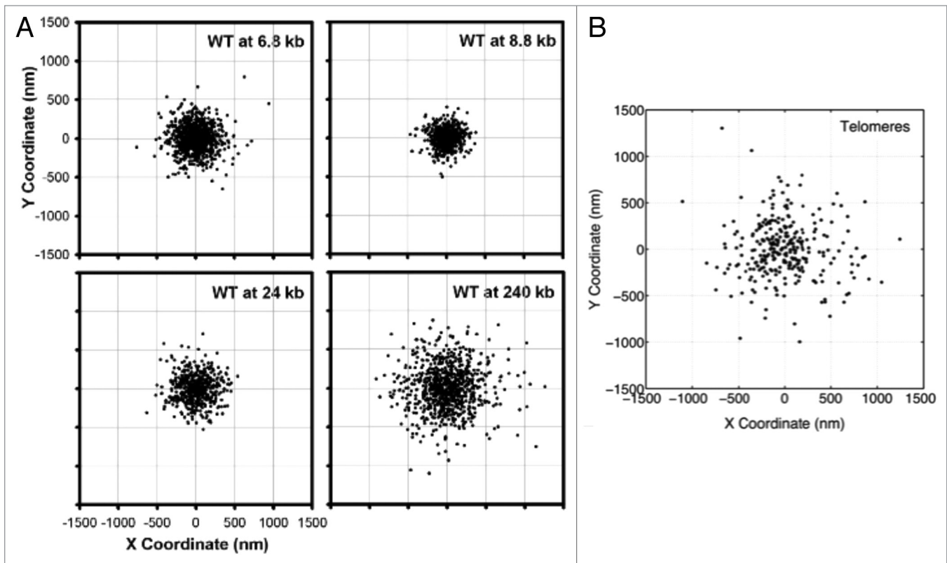
Figure 6. Scatter plots of loci positions, for (A) different locations within the chromosome arm and (B) telomere sites. (A) is adapted from reference 26. In a chromosome arm, the two extreme tethering points are the centromere and the telomere. Behavior of the telomere is fundamentally different from that of the centromere, implying different dynamics governing each site.
