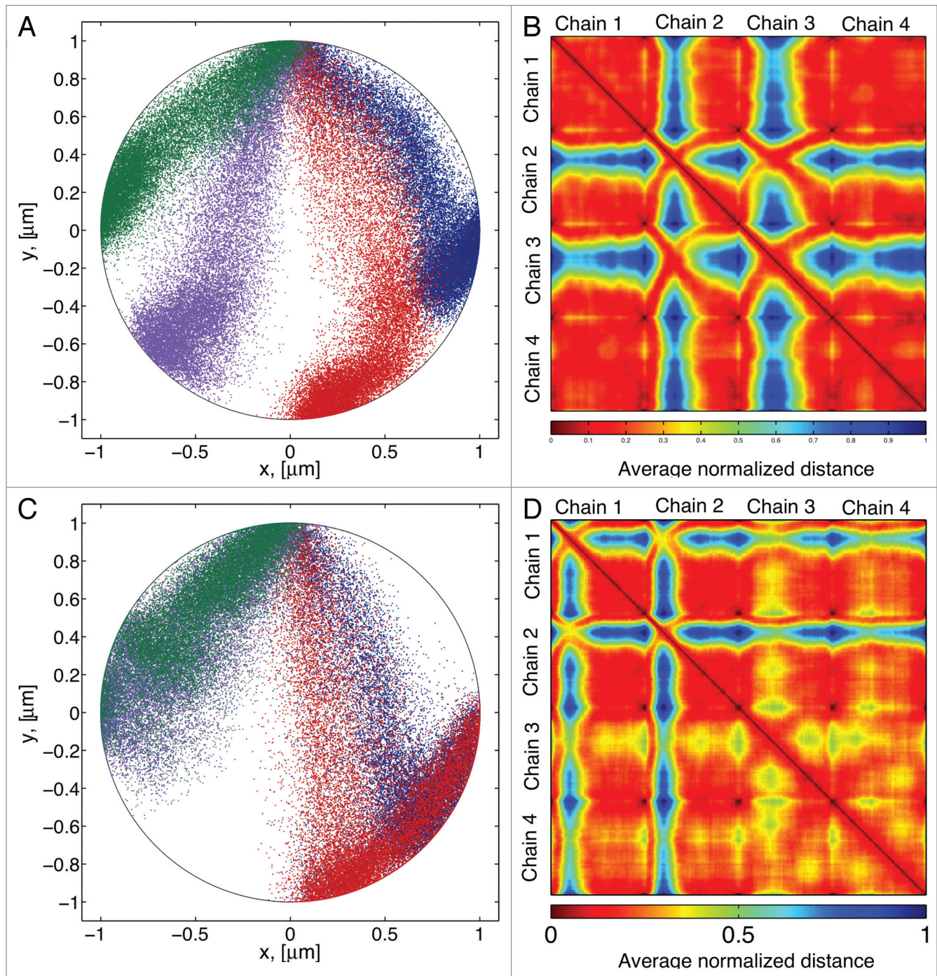
Figure 7. (A) Distribution of bead positions for chains tethered at different points in the cell boundary. Tether sites are located at \pi/2 , 3\pi/4 , 5\pi/4 , and 3\pi/2 in the circumference. (B) Interaction heat maps corresponding to bead positions in A, dark red corresponds small separations between beads (contact), blue corresponds to the maximum separation observed between two beads (no contact). (C) Distribution of bead positions when two chains are tethered at the same point. (D) Interaction heat map corresponding to (C).
