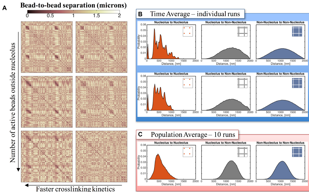
Figure 8. Distribution of bead-to-bead distances for split nucleolus. (A) Contact maps show that there is a marked increase in bead interactions within the nucleolus as a function of decreasing the on/off times of binding (left to right). Faster (weak) kinetics results in more interactions. Left column t_{on} = 0.09 s, right column t_{on} = 90 s. Active beads outside the nucleolus are introduced to account for binding interactions throughout the nucleus. In the non-nucleolar chromatin, interactive beads are inactive outside the nucleolus (stride zero—top row), every tenth bead is active (stride 10) and every third bead is active (stride 3—bottom row). (B) Sub-structures within the nucleolus are formed by clusters of beads that are closer, interact more frequently and maintain some separation between clusters. These fluctuating sub-structures create darker regions in the contact maps and peaks in the bead-bead proximity histograms within the nucleolus. Although dynamic, these sub-structures persist over time for a given run (see Supplementary Movie 3) and are robust from run-to-run although the nucleolar bead cluster assignments are random. Top and bottom panels correspond to the same model parameters but different random seed. (C) The sub-structures are lost in the population averages, even though the cluster morphology is robust, because of random cluster assignments, resulting in a more uniform distribution of bead-to-bead distances within the nucleolus. X- and Y-axis for each contact map correspond to bead numbers, as explained in Figure 4.
