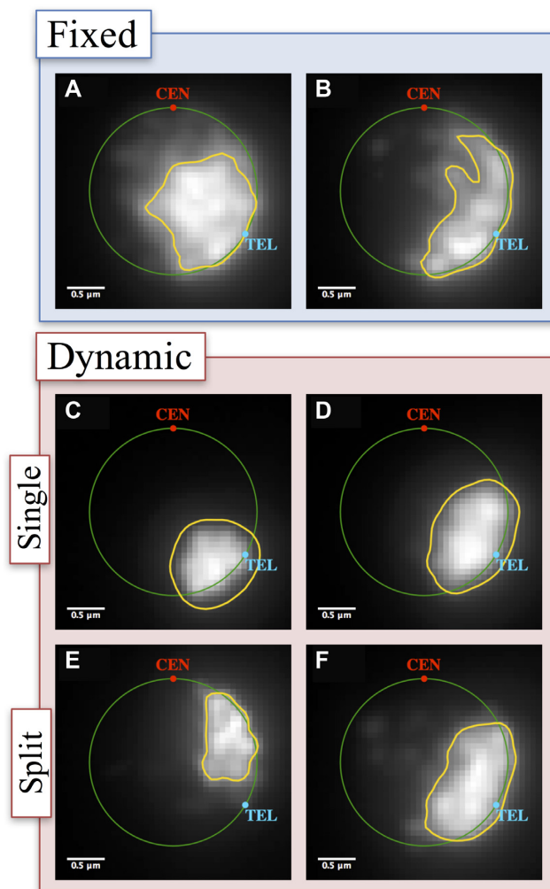
Figure 3. Qualitative analysis of nucleolus area. Simulation results converted to microscope images (see ‘Materials and Methods’ section). (A) Without crosslinks, (B) uniform, fixed cross-links, (C) dynamic crosslinks for single nucleolus with t_{\text{on}} = 0.09 s, (D) dynamic crosslinks for single nucleolus with t_{\text{on}} = 90 s, (E) dynamic crosslinks for split nucleolus with t_{\text{on}} = 0.09 s and (F) dynamic crosslinks for split nucleolus with t_{\text{on}} = 90 s.
