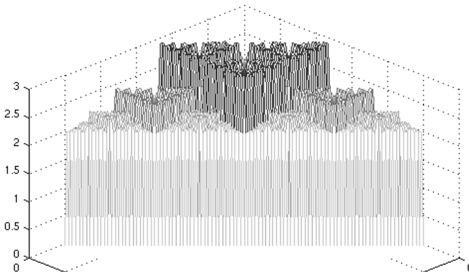
FIGURE 2. Graph of z = E(x, y, 1 - x - y) for 0 \leq x \leq 1 - y \leq 1
