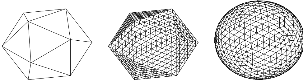
FIGURE 2. Partitioning a sphere.
