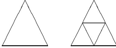
FIGURE 1. Subdividing a triangle.
