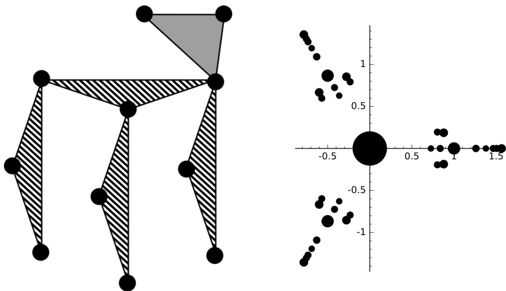
Figure 1: \mathcal{H}_3 and its spectrum.
