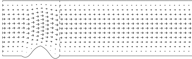
Figure 7.2: Locally minimizing flow produced by the optimizer. The global minimizer has a parabolic bump, and no “gutters”.
