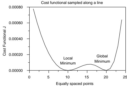
Figure 7.1: The functional between local and global minimizers. The local minimizer has J_2 = 0.3E - 06 , the global minimizer has J_2 = 0 .
