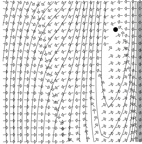
Figure 9.6: Gradients approximated by sensitivities. The approximate gradients clearly do not match the contours.
