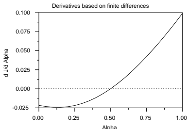
Figure 9.5: \frac{dJ_2}{d\alpha} by finite differences and sensitivities. The two calculations are now essentially identical.
