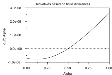
Figure 9.2: \frac{dJ}{d\alpha} by finite differences.
