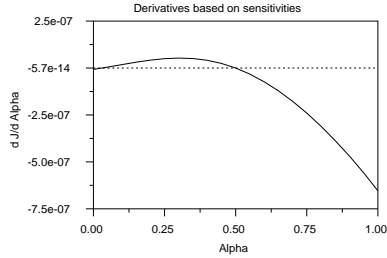
Figure 9.3: \frac{dJ_1}{d\alpha} by sensitivities.
