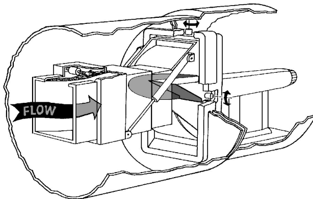
Figure 1.1: An aircraft engine and forebody simulator in a wind tunnel.
