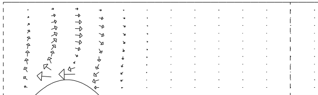
Figure 6.1: Derivatives of the velocity with respect to the bump parameter.
