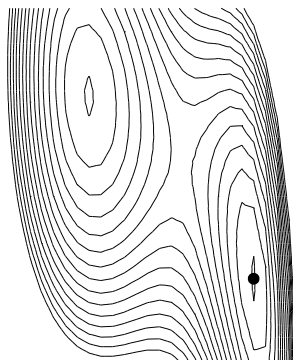
Figure 7.3: Contours for J_2 on plane including local and global minima. The global minimum is marked.
