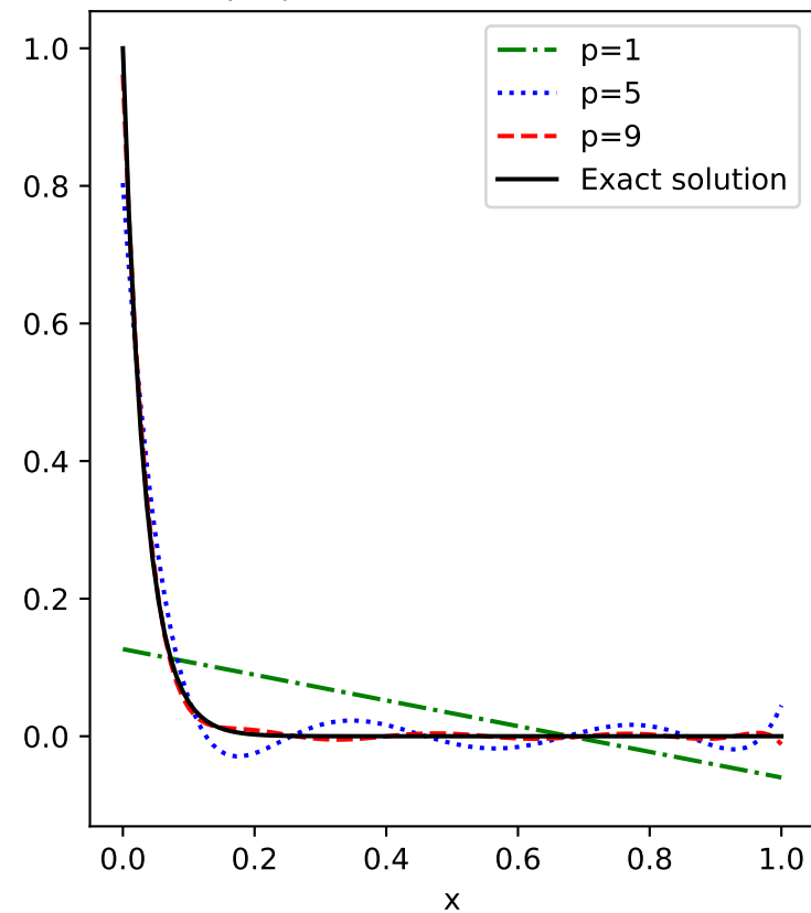
L^2 projections of exact solution
