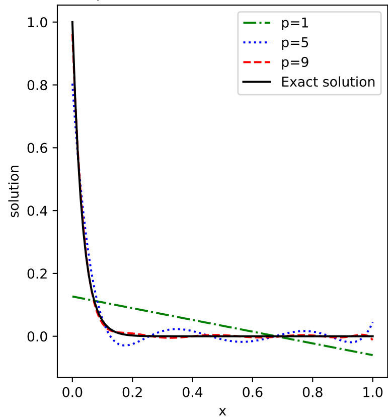
Spectral Petrov-Galerkin solutions
