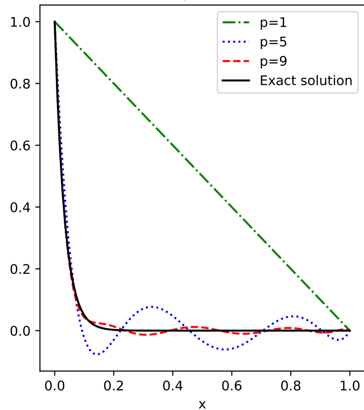
L^2 Least-Squares solutions
