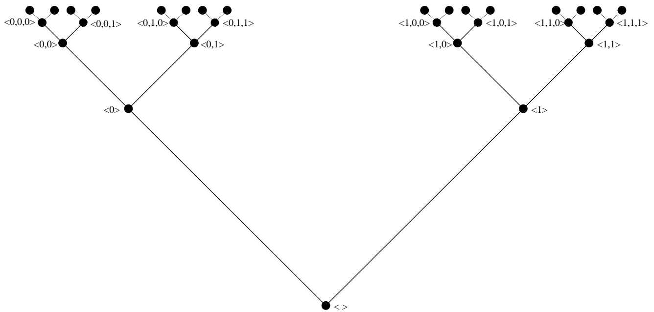
Fig. 1 The Cantor tree (or the Cantor road space depending on how you interpret it).
